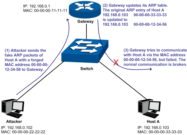
Figure 12-12 ARP Attack – Cheating Gateway
