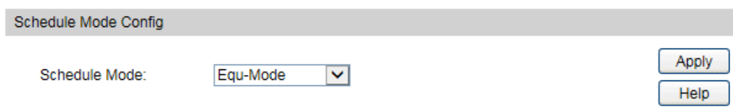
Figure 9-7 Schedule Mode
