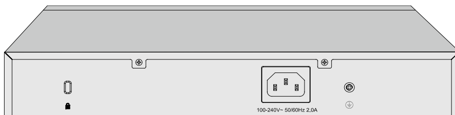
Figure 2-4 Rear Panel of the switch
